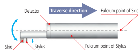
Measuring example of stepped features: Skidded
