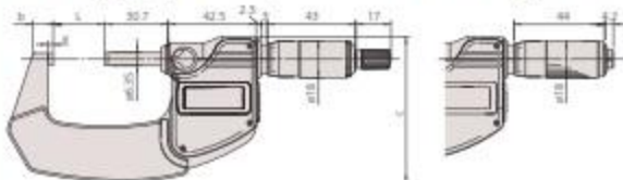
Ratchet stop type (up to 100mm/4")
