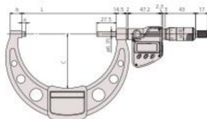
Ratchet stop type (over 100mm/4" to 300mm/12")
