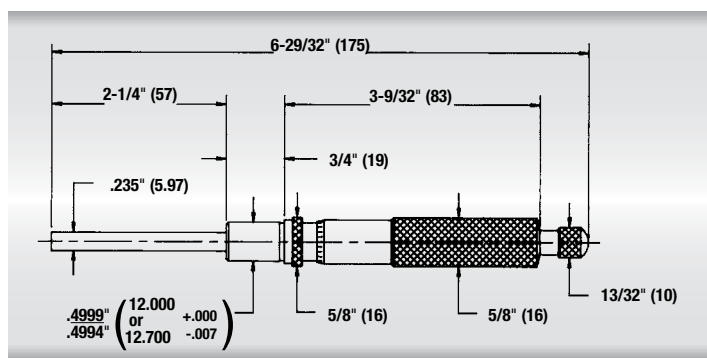
63RL, 0-2" and 63MRL (0-50 mm) dimensions
