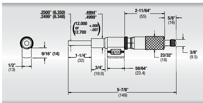
363RL, 0-1" and 363MRL (0-25mm) dimensions
