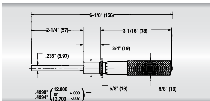
63P, 0-2" and 63MP (0-50mm) dimensions
