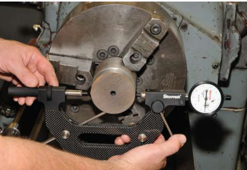
5003 Carbon Fiber Snap Gages
