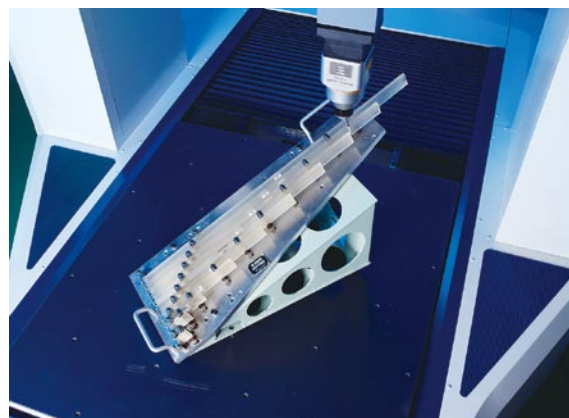
Figure 44 Calibration of a high-precision coordinate measuring machine with low-expansion glass gauge blocks
