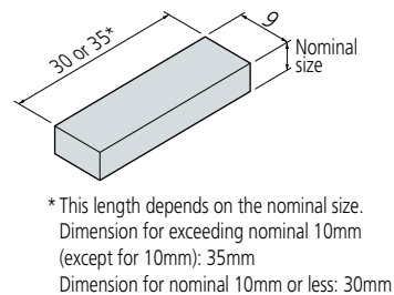
Figure 5 Johansson type (rectangular type) gauge block
