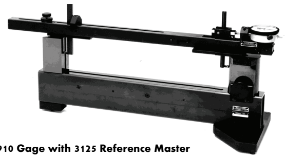
2910 Gage with 3125 Reference Master
