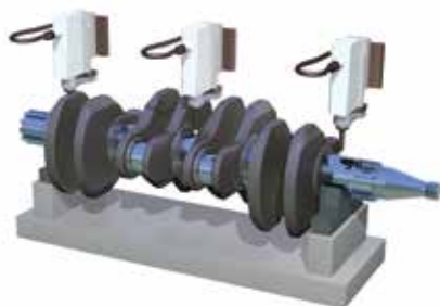
⑦ Workpiece runout measurement
