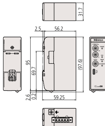
Interface unit CC-Link
