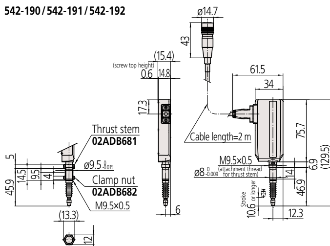
Dimensions with an optional thrust stem installed
