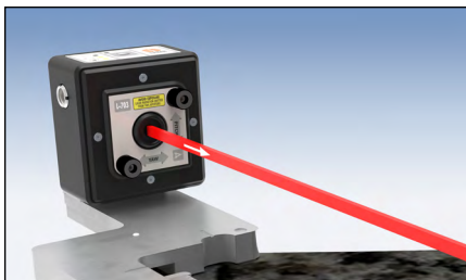
L-703SP Spindle and Straightness Laser
