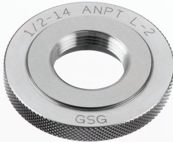
TAPER PIPE THREAD - RINGS - WORKING GAGES
