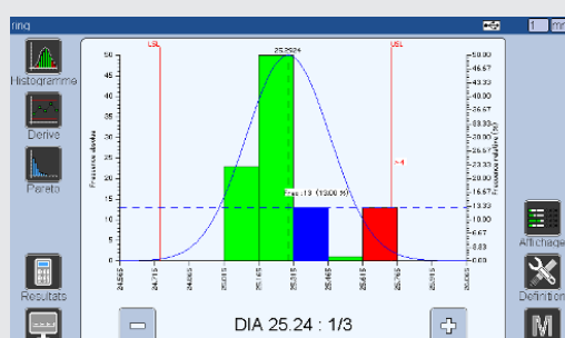
Histogram with Gaussian Curve
